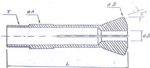
DRAW-IN TYPE COLLET
